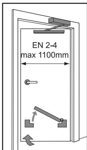
Transom mount push side
