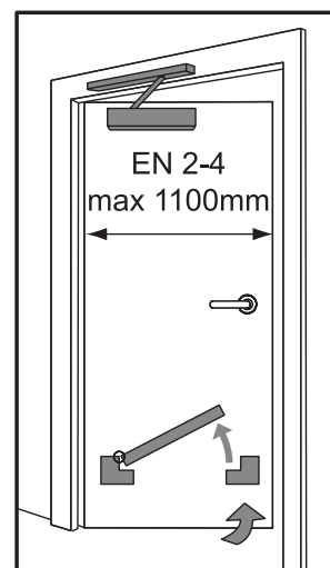
Door mount push side
