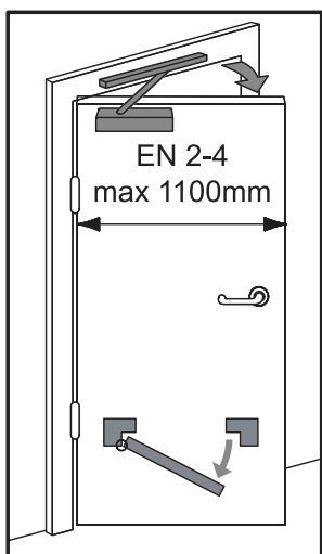
Door mount pull side
